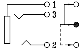
SCHMATIC (NON-SHORTING) ST-212-02V
