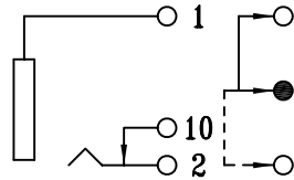
SCHMATIC (NON-SHORTING) ST-212-03V
