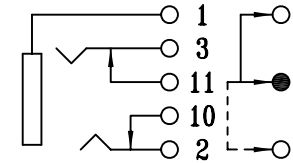
SCHMATIC (NON-SHORTING) ST-212-06V
